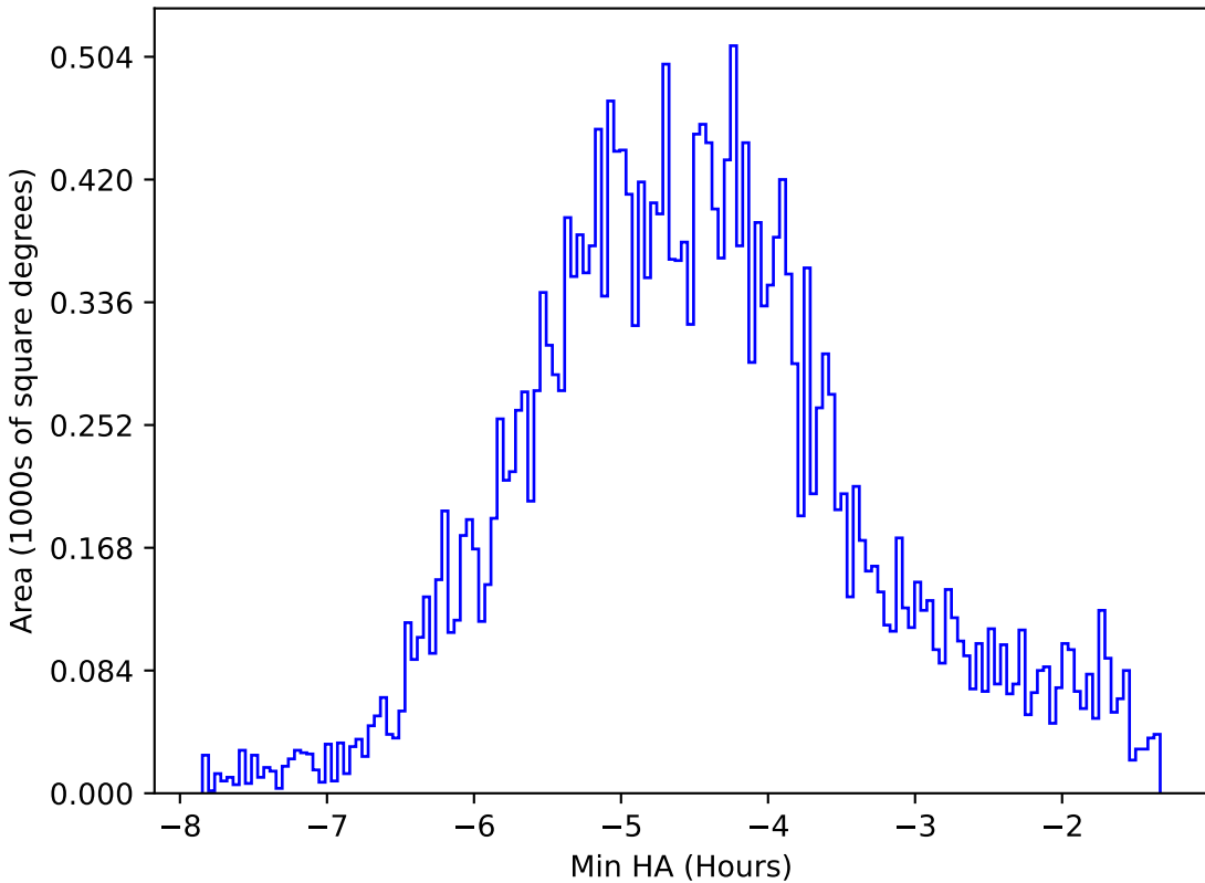
ddf_loaded_fl15_v3.4_10yrs All sky all bands: Min HA
