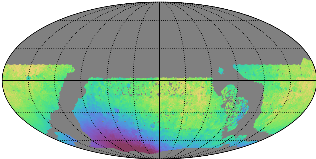
ddf_loaded_fl15_v3.4_10yrs WFD y band: Median solarElong
