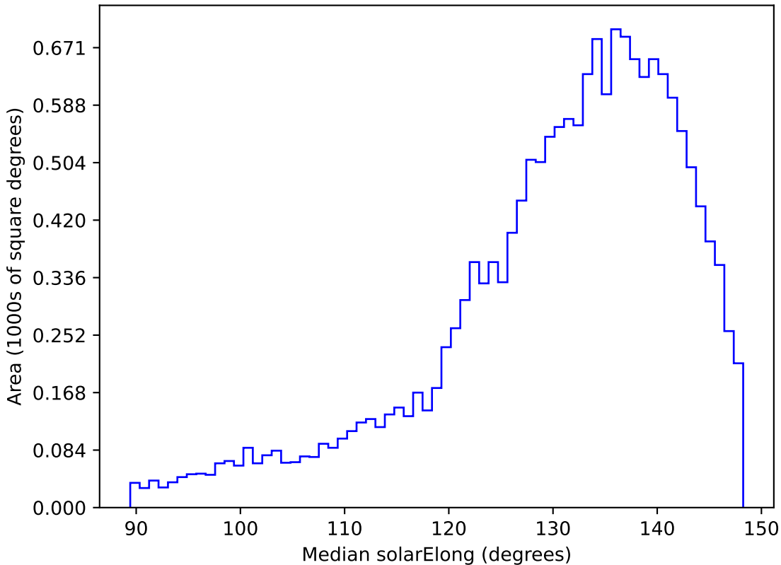
ddf_loaded_fl15_v3.4_10yrs WFD r band: Median solarElong
