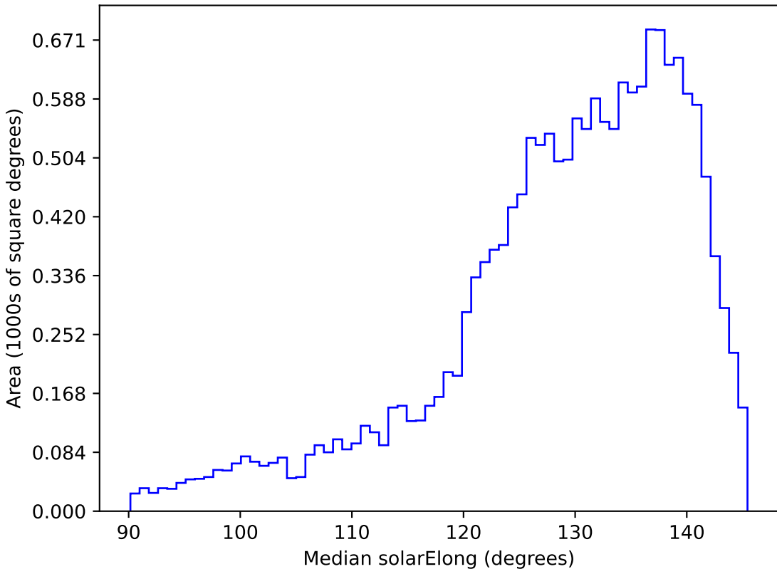
ddf_loaded_fl15_v3.4_10yrs WFD i band: Median solarElong
