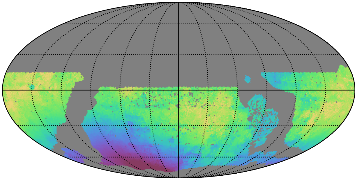
ddf_loaded_fl15_v3.4_10yrs WFD g band: Median solarElong
