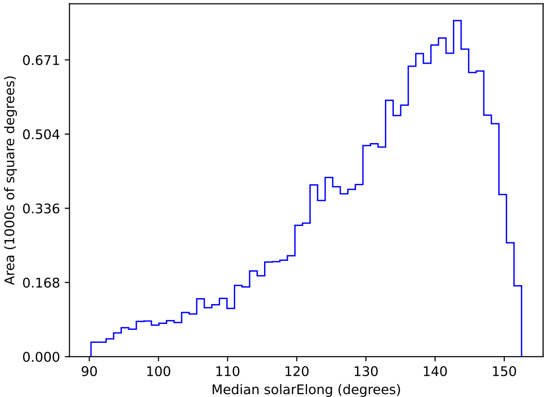
ddf_loaded_fl15_v3.4_10yrs WFD g band: Median solarElong
