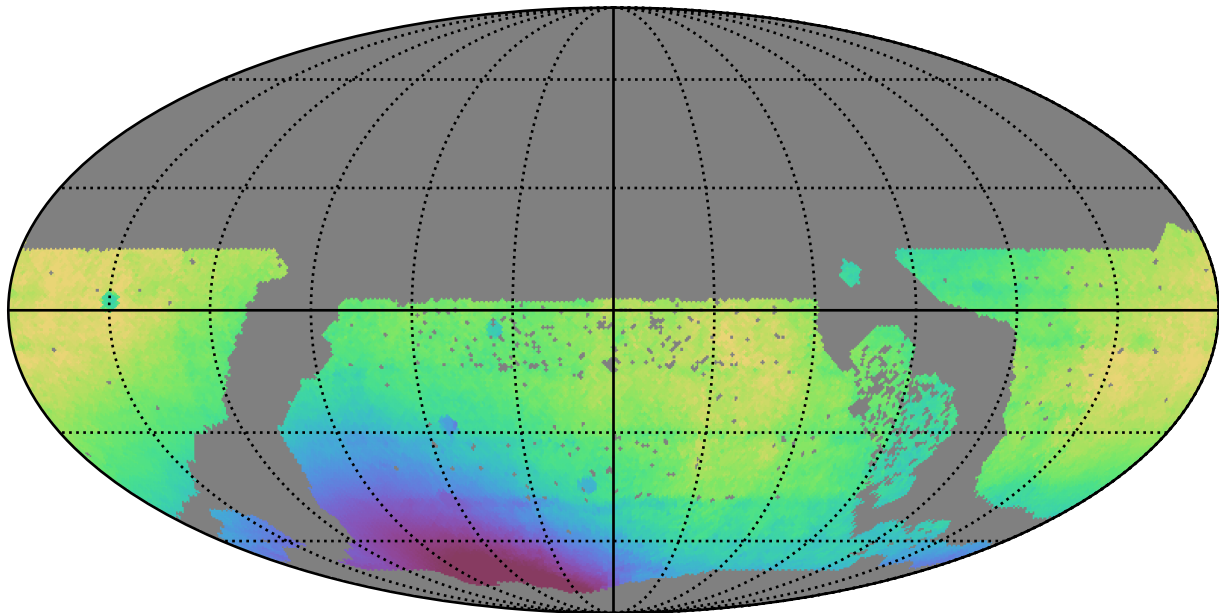
ddf_loaded_fl15_v3.4_10yrs WFD all bands: Median solarElong
