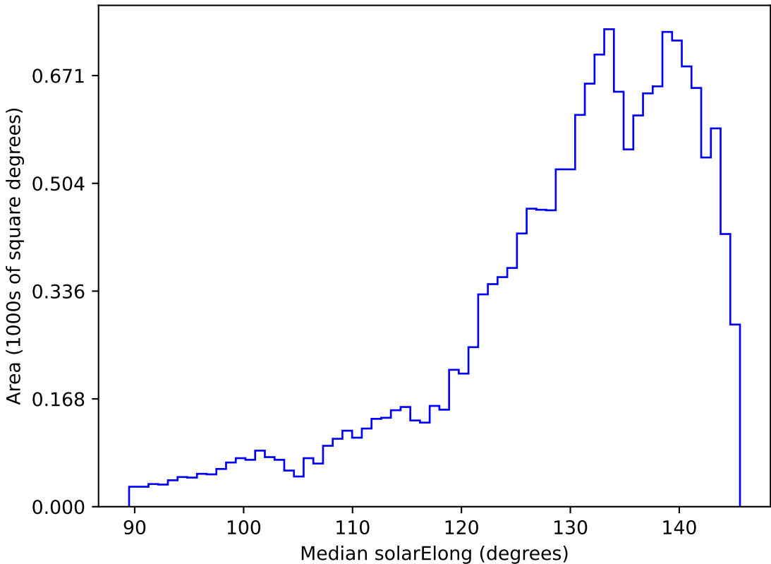
ddf_loaded_fl15_v3.4_10yrs WFD all bands: Median solarElong
