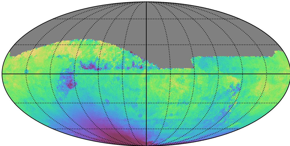
ddf_loaded_fl15_v3.4_10yrs All sky z band: Median solarElong
