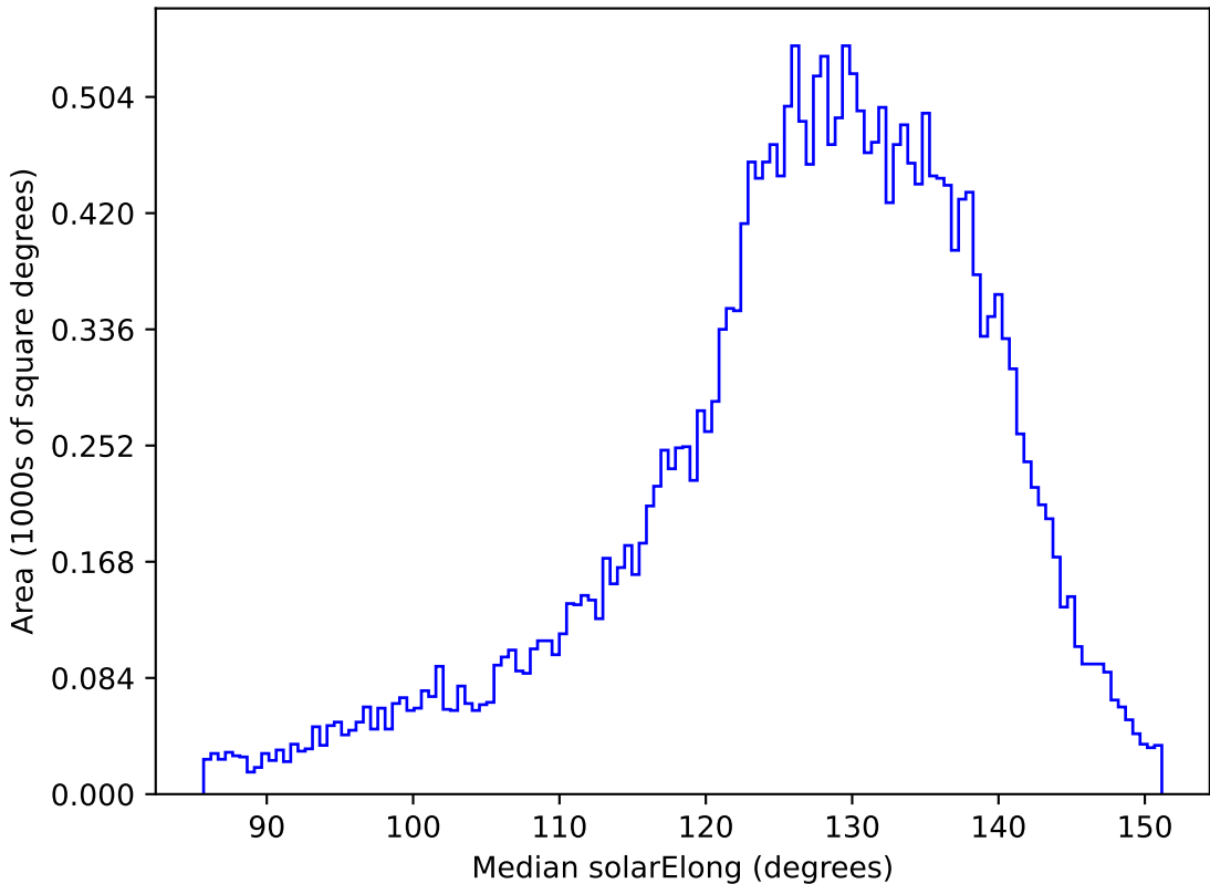
ddf_loaded_fl15_v3.4_10yrs All sky z band: Median solarElong
