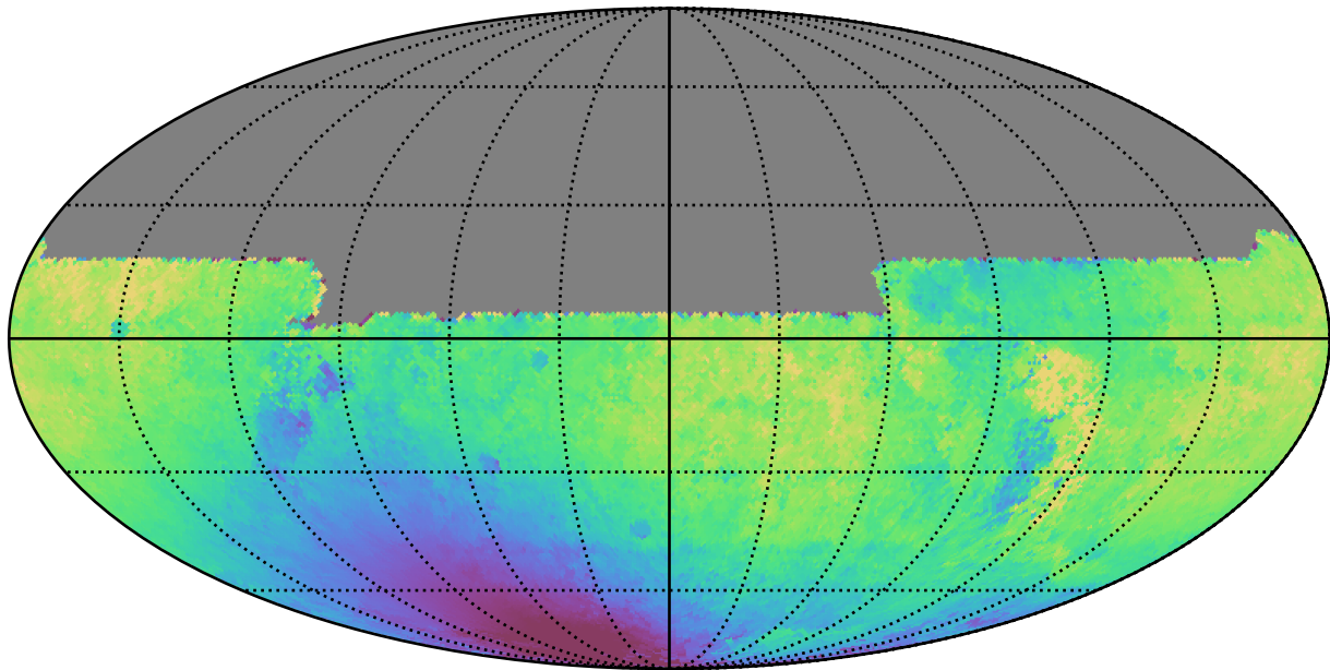
ddf_loaded_fl15_v3.4_10yrs All sky y band: Median solarElong
