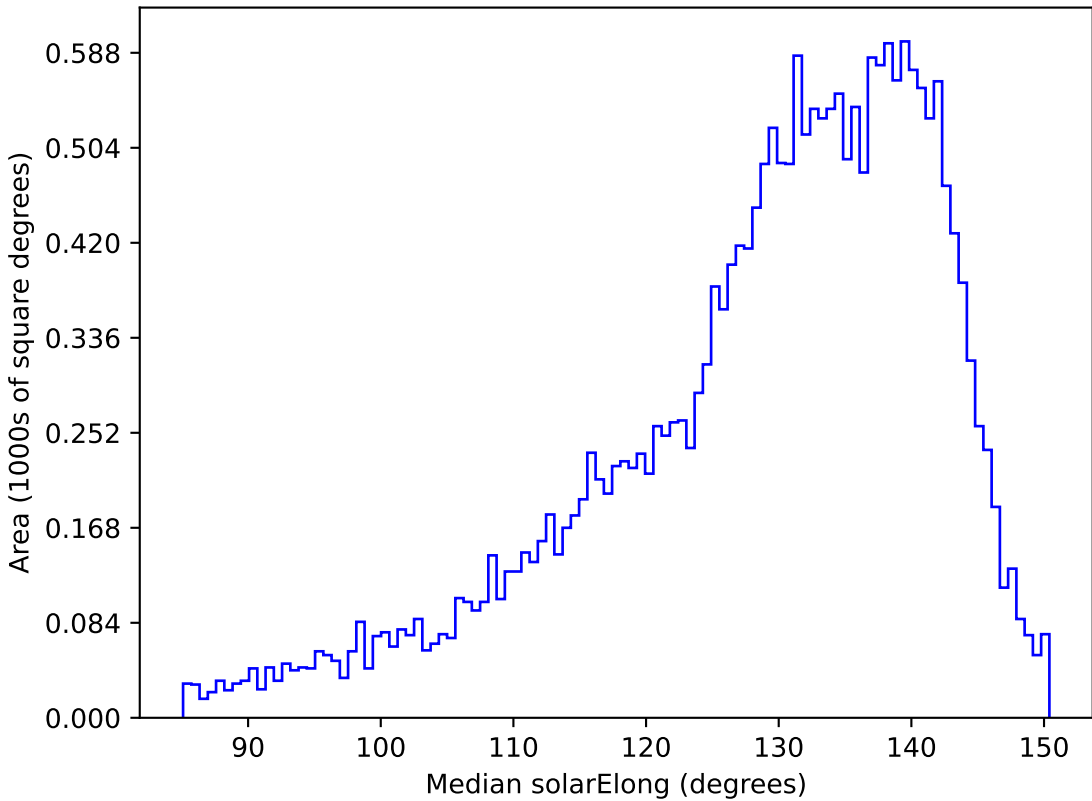
ddf_loaded_fl15_v3.4_10yrs All sky y band: Median solarElong
