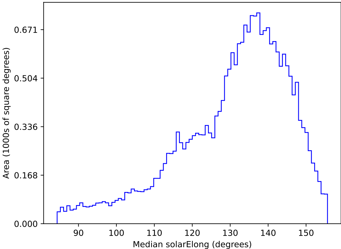
ddf_loaded_fl15_v3.4_10yrs All sky u band: Median solarElong
