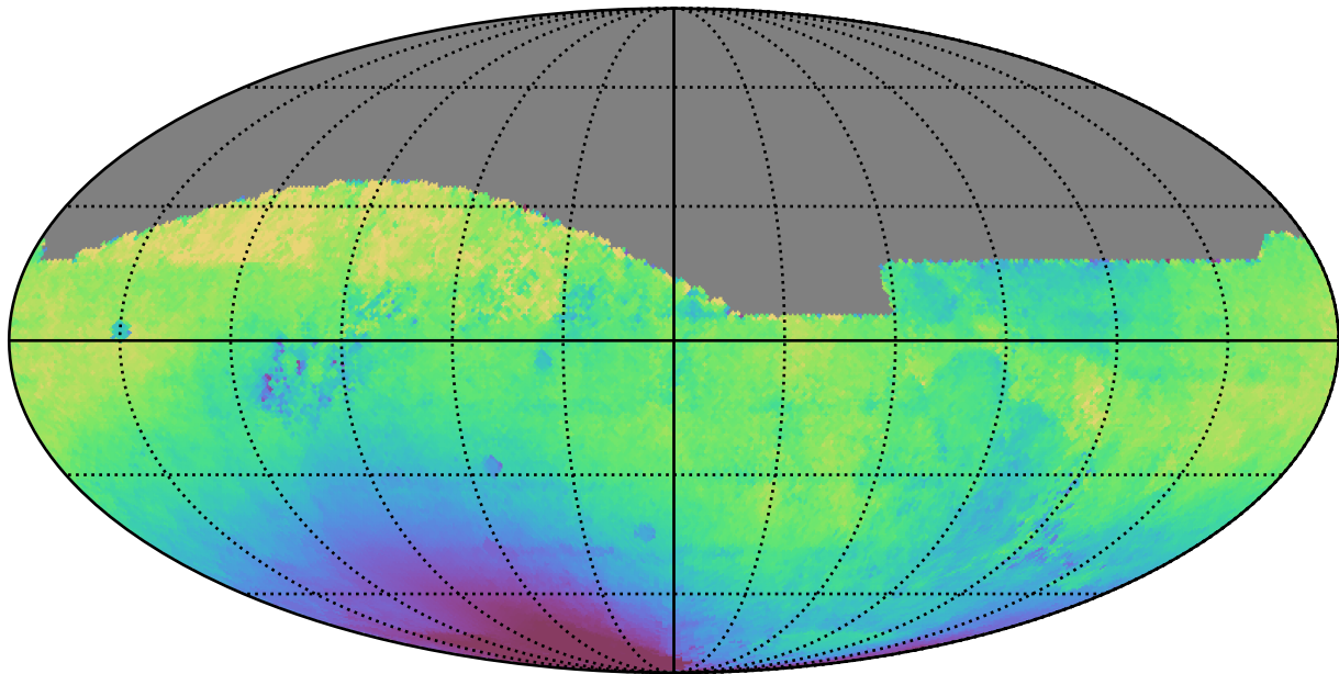
ddf_loaded_fl15_v3.4_10yrs All sky r band: Median solarElong
