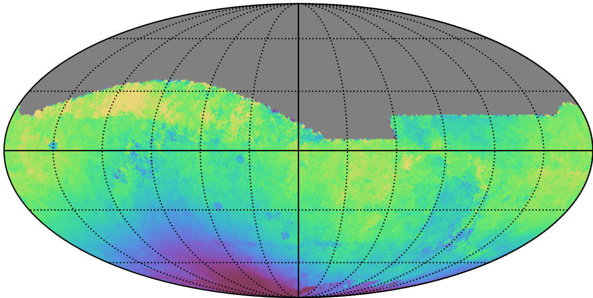
ddf_loaded_fl15_v3.4_10yrs All sky i band: Median solarElong
