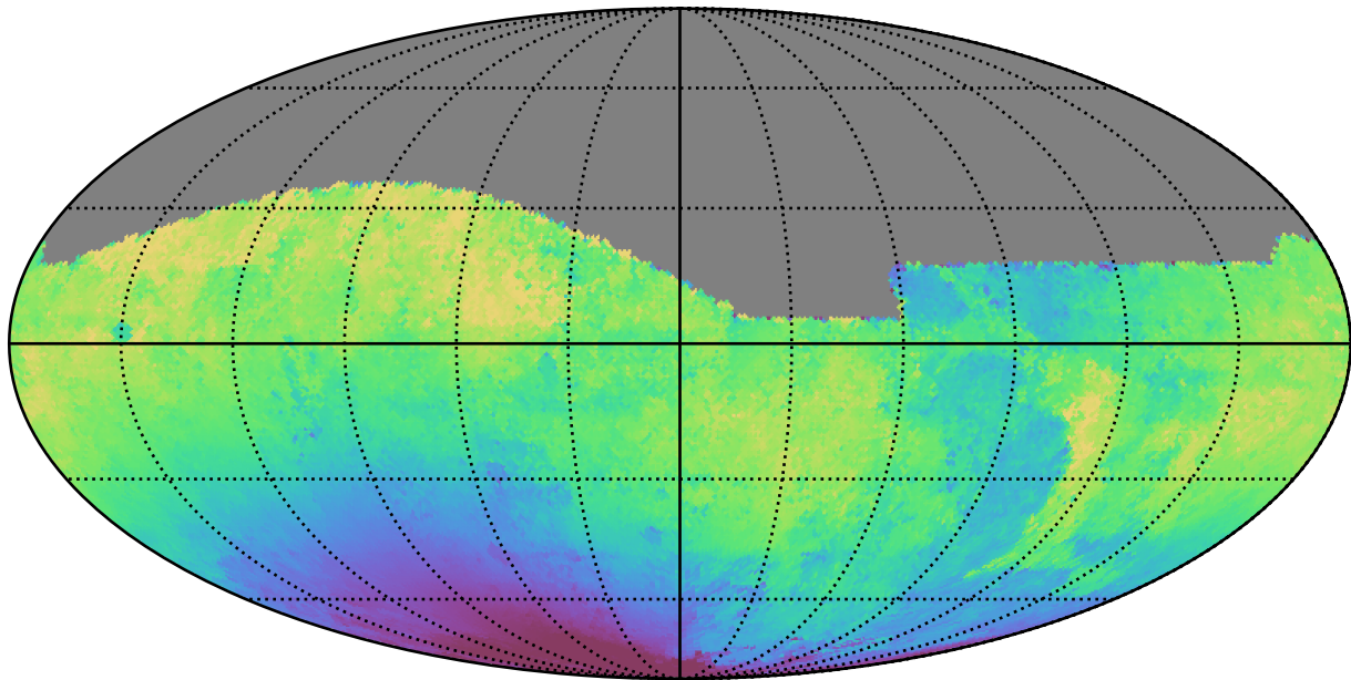
ddf_loaded_fl15_v3.4_10yrs All sky g band: Median solarElong
