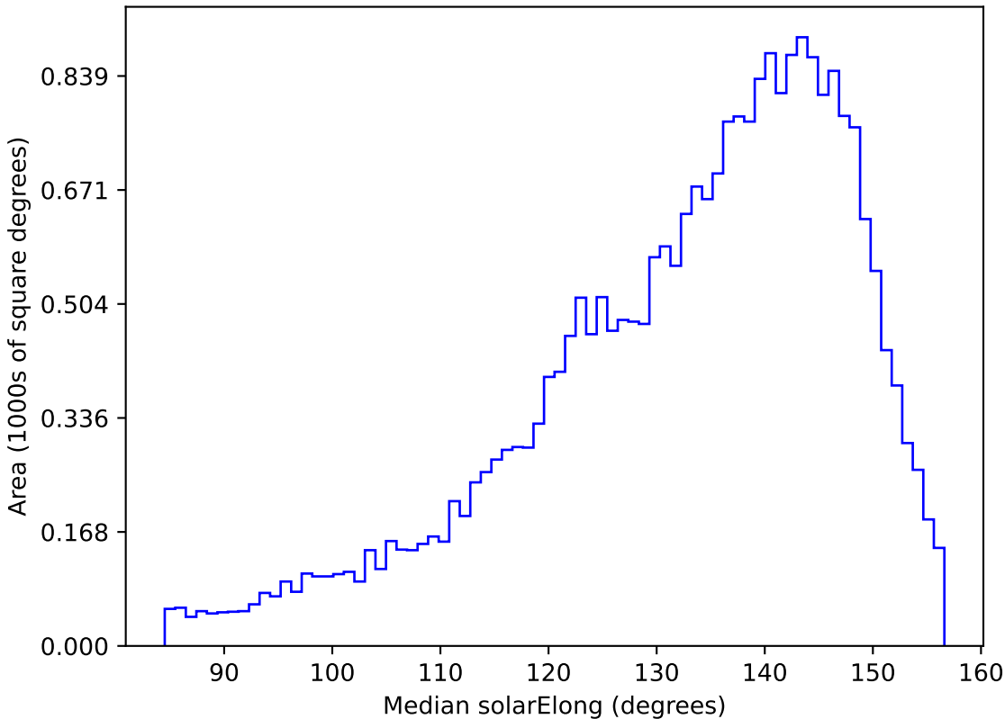
ddf_loaded_fl15_v3.4_10yrs All sky g band: Median solarElong
