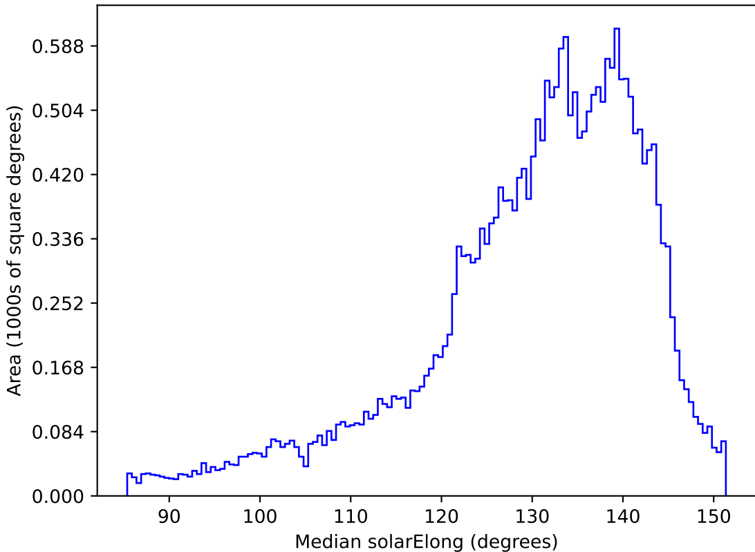
ddf_loaded_fl15_v3.4_10yrs All sky all bands: Median solarElong
