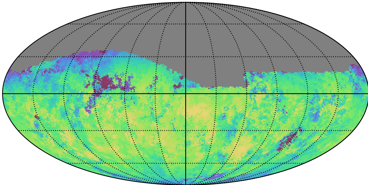
ddf_loaded_fl15_v3.4_10yrs Yr 1 z band: Median skyBrightness
