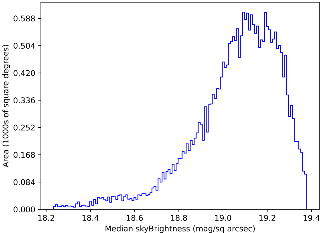
ddf_loaded_fl15_v3.4_10yrs Yr 1 z band: Median skyBrightness
