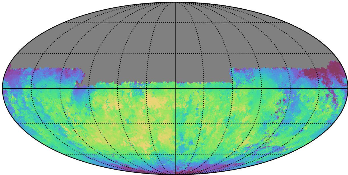
ddf_loaded_fl15_v3.4_10yrs Yr 1 y band: Median skyBrightness
