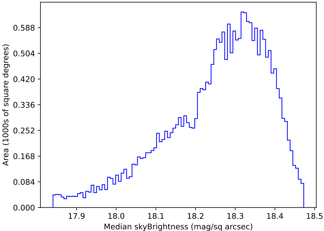
ddf_loaded_fl15_v3.4_10yrs Yr 1 y band: Median skyBrightness
