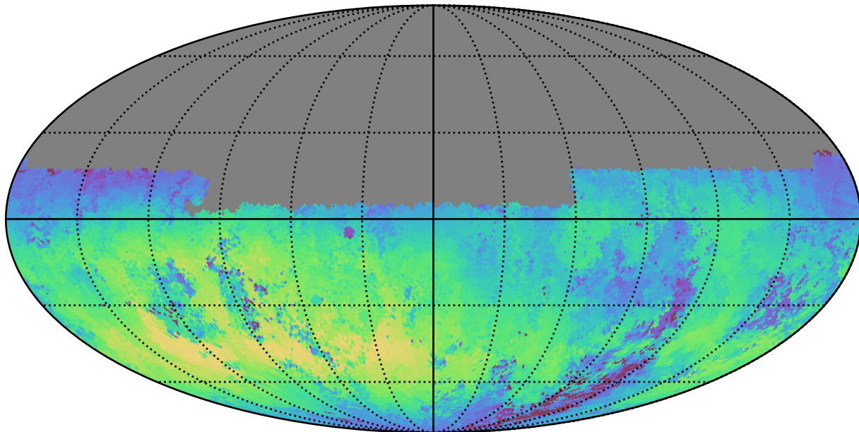
ddf_loaded_fl15_v3.4_10yrs Yr 1 u band: Median skyBrightness
