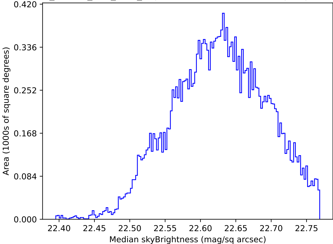
ddf_loaded_fl15_v3.4_10yrs Yr 1 u band: Median skyBrightness
