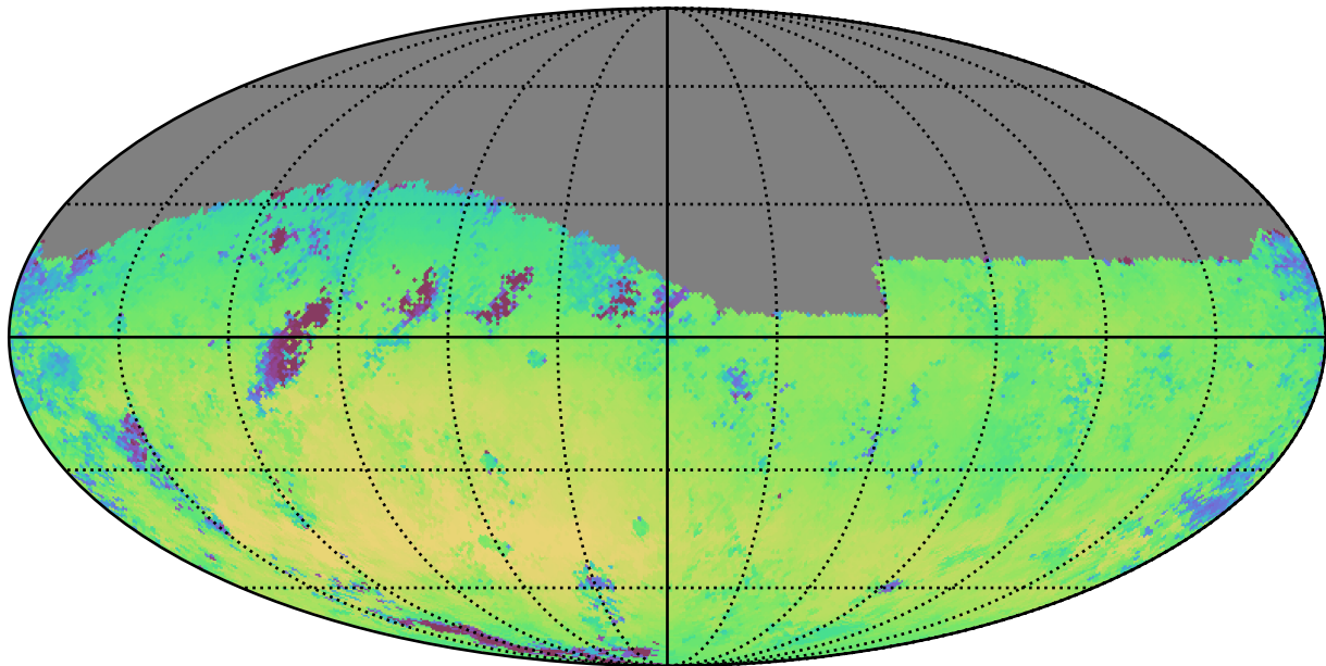
ddf_loaded_fl15_v3.4_10yrs Yr 1 r band: Median skyBrightness
