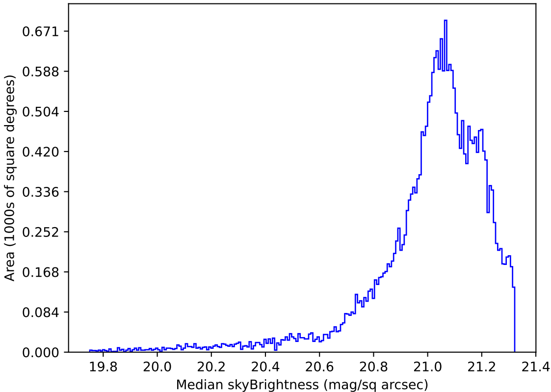
ddf_loaded_fl15_v3.4_10yrs Yr 1 r band: Median skyBrightness
