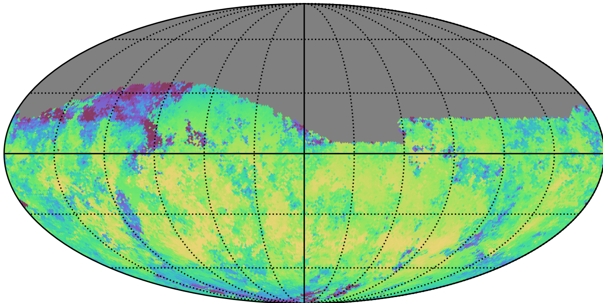
ddf_loaded_fl15_v3.4_10yrs Yr 1 i band: Median skyBrightness
