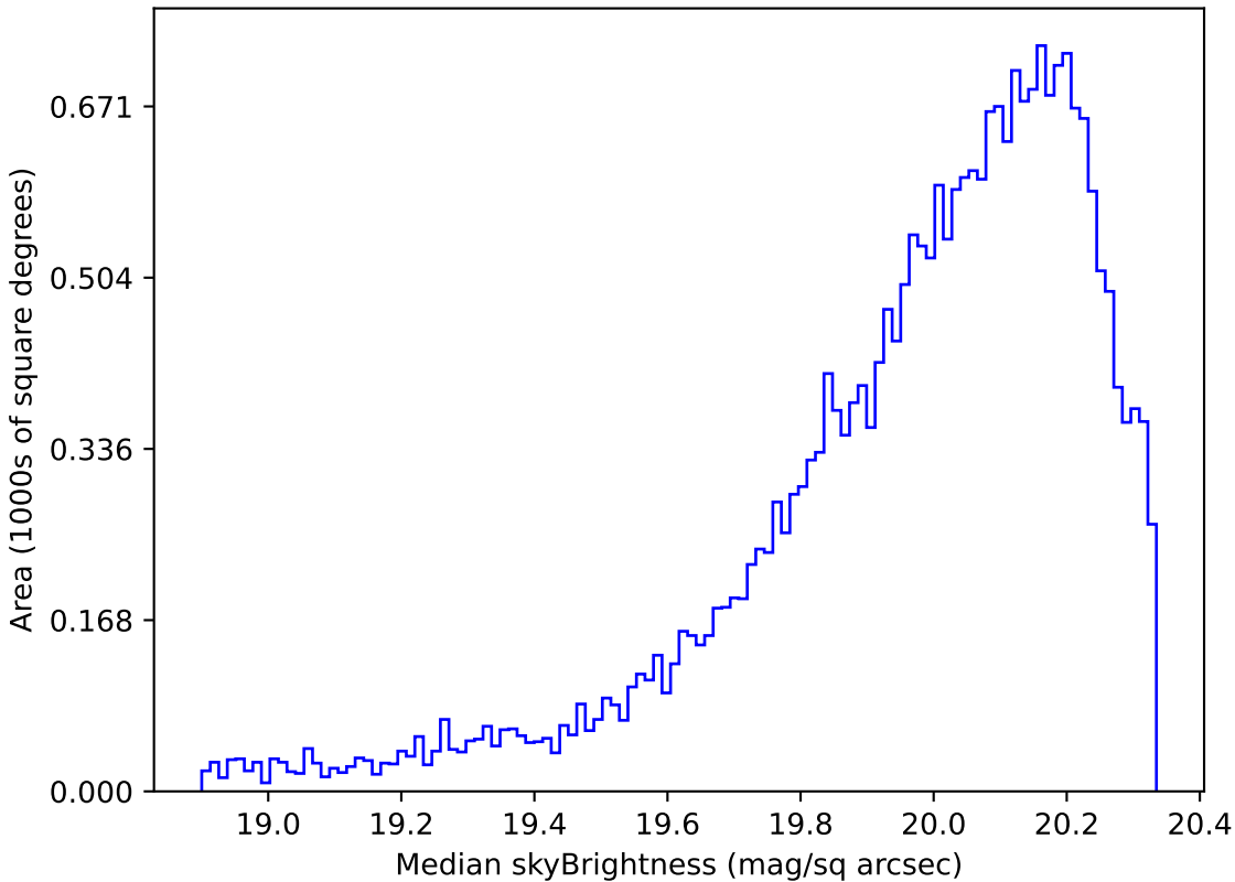
ddf_loaded_fl15_v3.4_10yrs Yr 1 i band: Median skyBrightness
