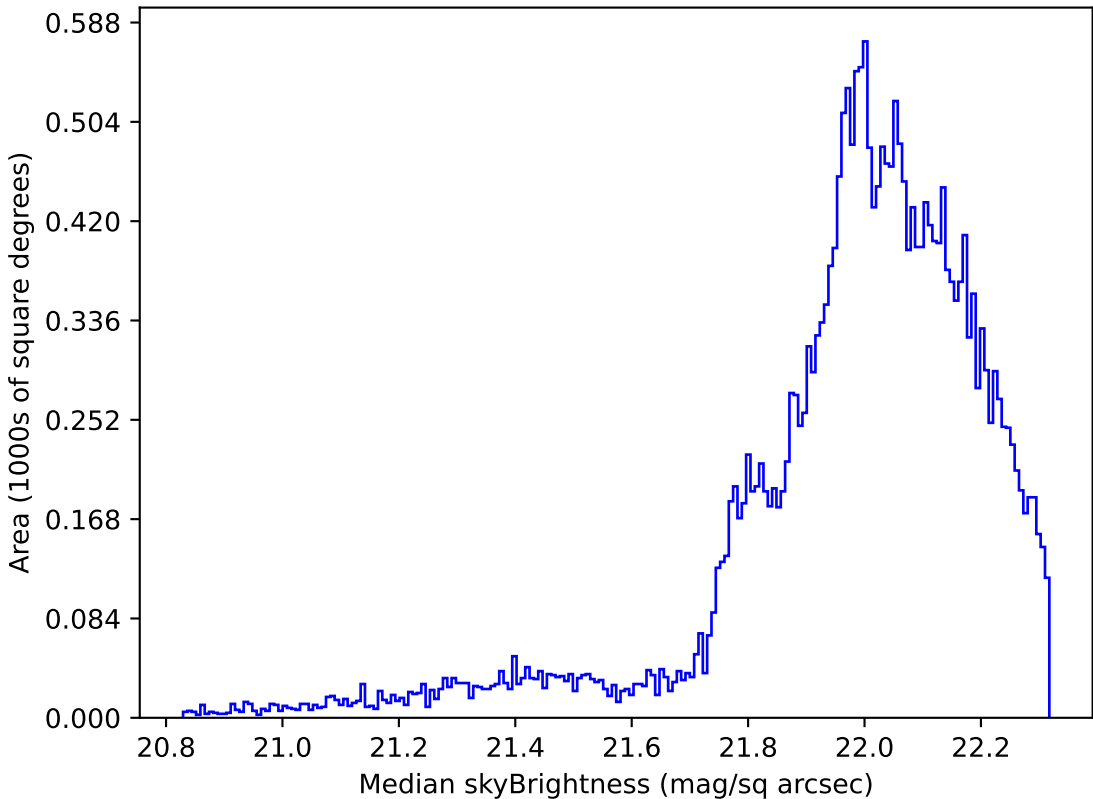
ddf_loaded_fl15_v3.4_10yrs Yr 1 g band: Median skyBrightness
