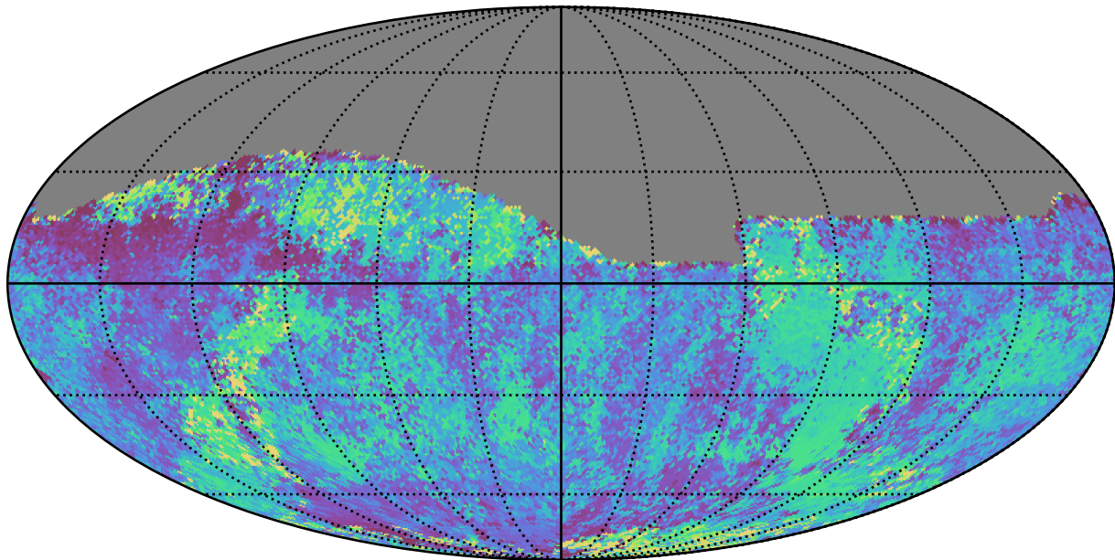
ddf_loaded_fl15_v3.4_10yrs Yr 1 all bands: Median skyBrightness
