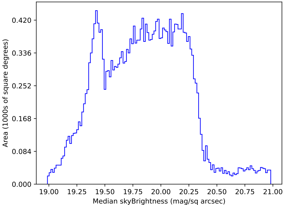
ddf_loaded_fl15_v3.4_10yrs Yr 1 all bands: Median skyBrightness
