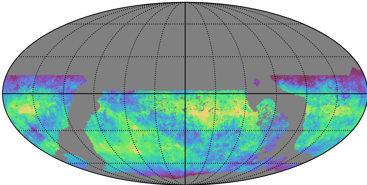
ddf_loaded_fl15_v3.4_10yrs WFD z band: Median skyBrightness
