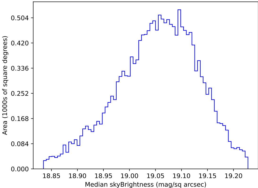
ddf_loaded_fl15_v3.4_10yrs WFD z band: Median skyBrightness
