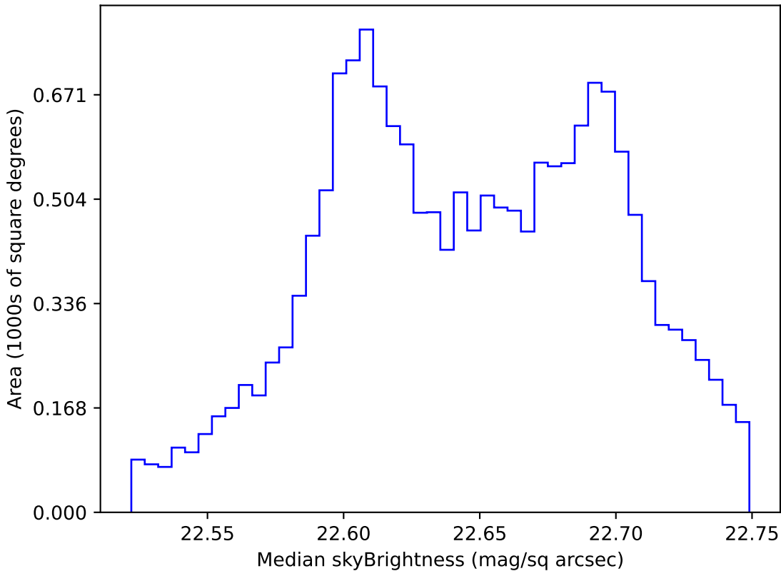
ddf_loaded_fl15_v3.4_10yrs WFD u band: Median skyBrightness
