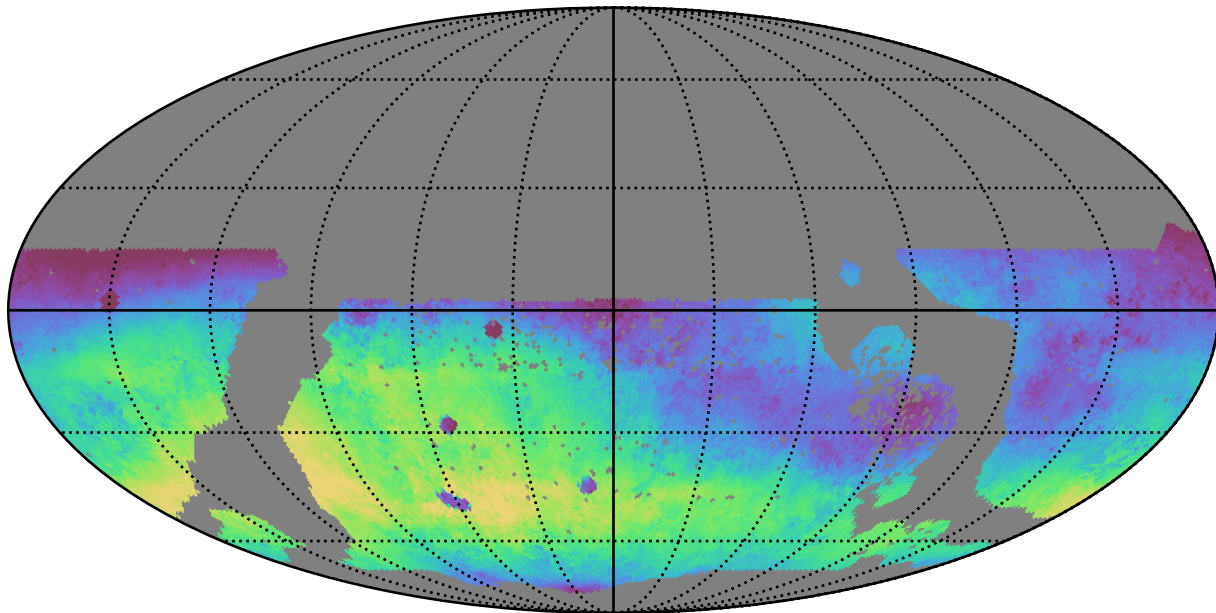
ddf_loaded_fl15_v3.4_10yrs WFD r band: Median skyBrightness
