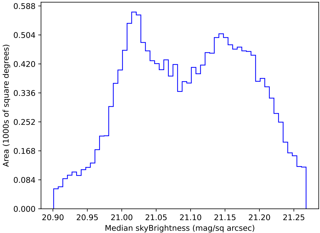
ddf_loaded_fl15_v3.4_10yrs WFD r band: Median skyBrightness
