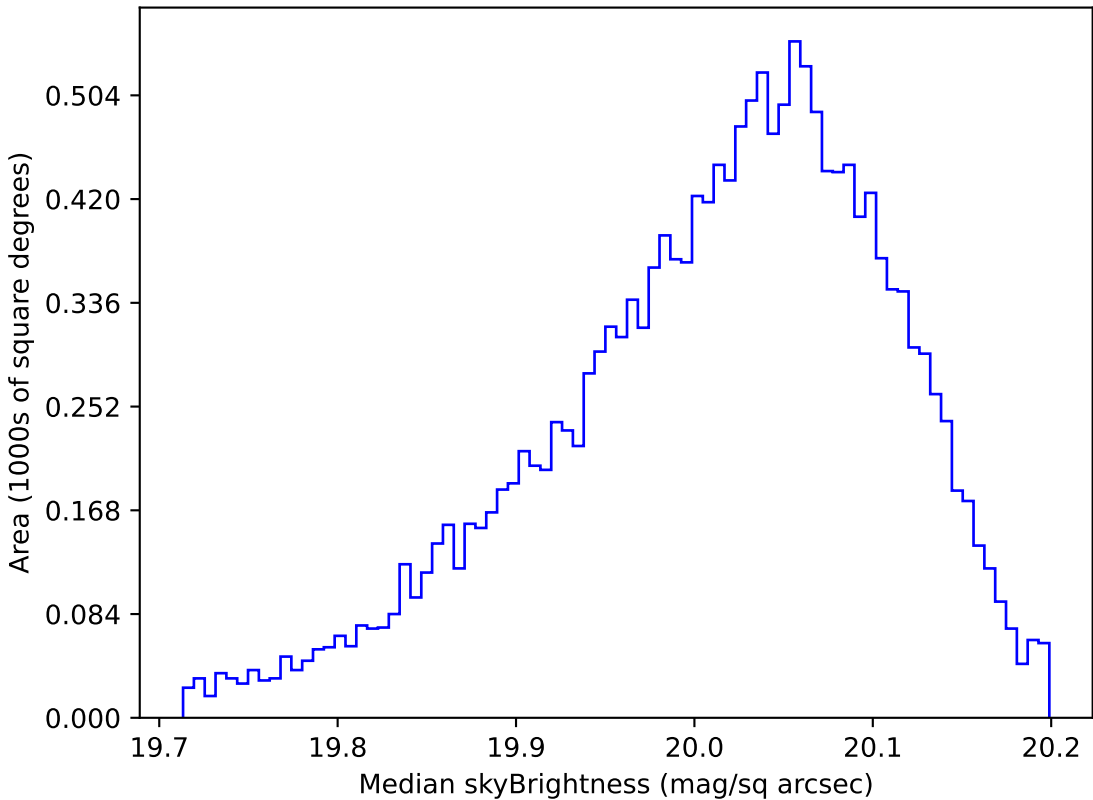
ddf_loaded_fl15_v3.4_10yrs WFD i band: Median skyBrightness
