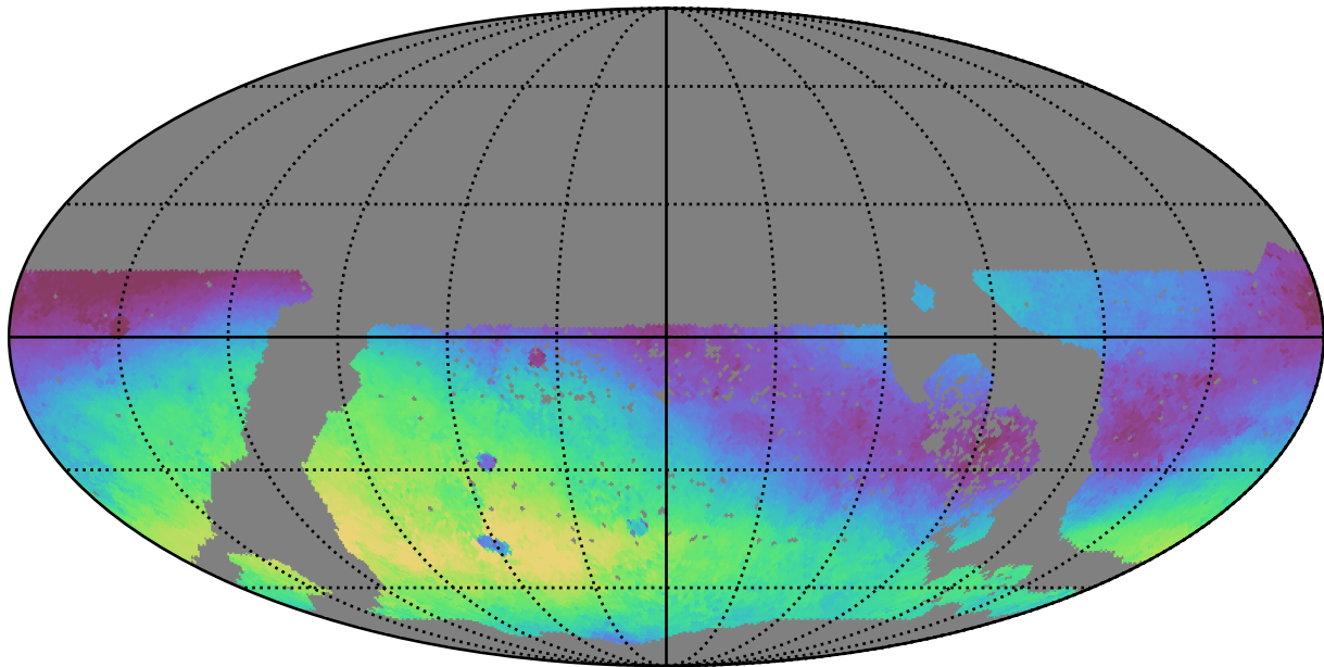
ddf_loaded_fl15_v3.4_10yrs WFD g band: Median skyBrightness
