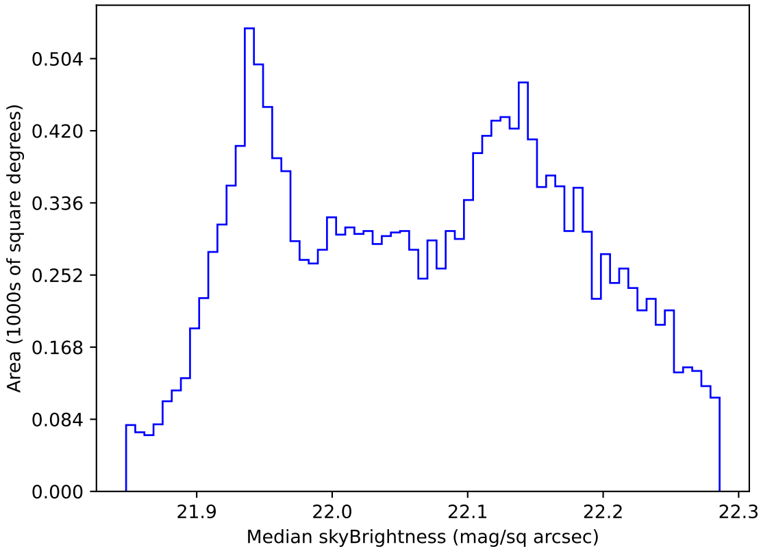
ddf_loaded_fl15_v3.4_10yrs WFD g band: Median skyBrightness
