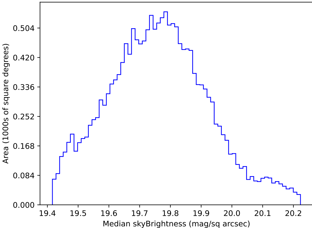
ddf_loaded_fl15_v3.4_10yrs WFD all bands: Median skyBrightness
