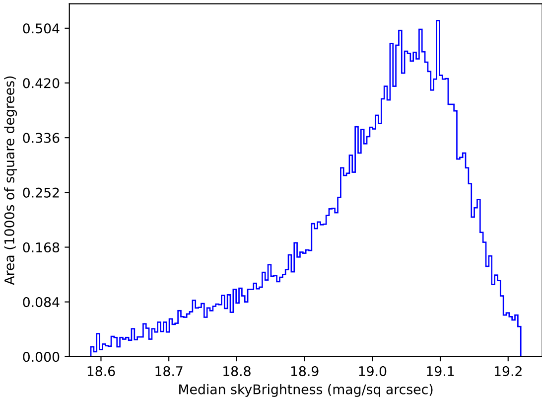
ddf_loaded_fl15_v3.4_10yrs All sky z band: Median skyBrightness
