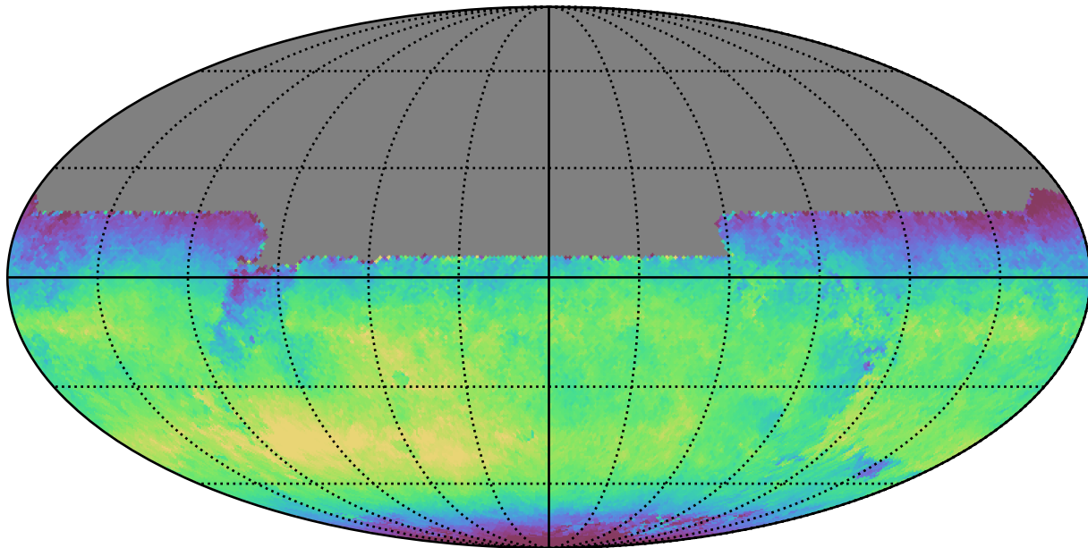
ddf_loaded_fl15_v3.4_10yrs All sky y band: Median skyBrightness
