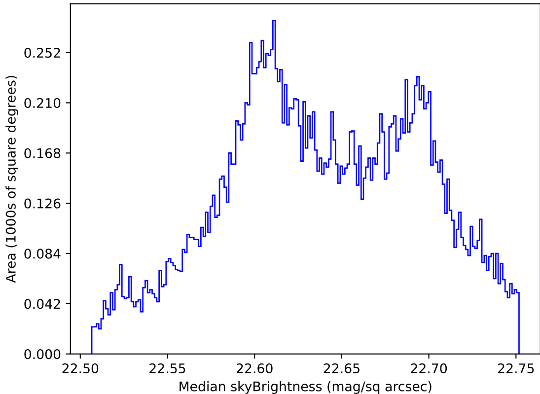
ddf_loaded_fl15_v3.4_10yrs All sky u band: Median skyBrightness
