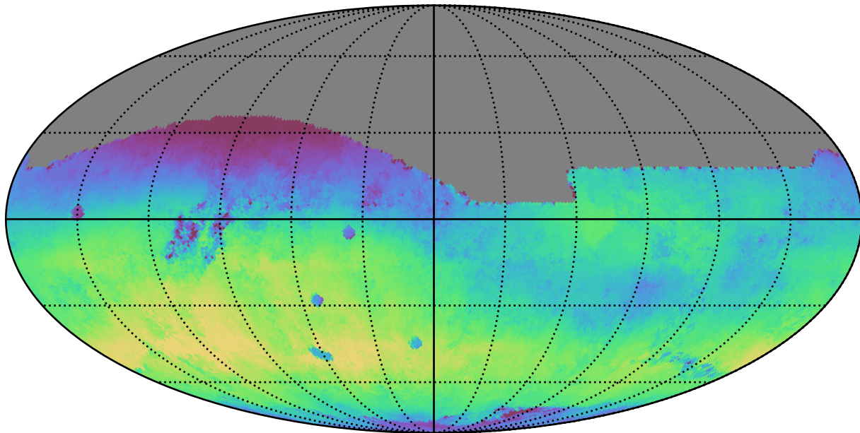
ddf_loaded_fl15_v3.4_10yrs All sky r band: Median skyBrightness
