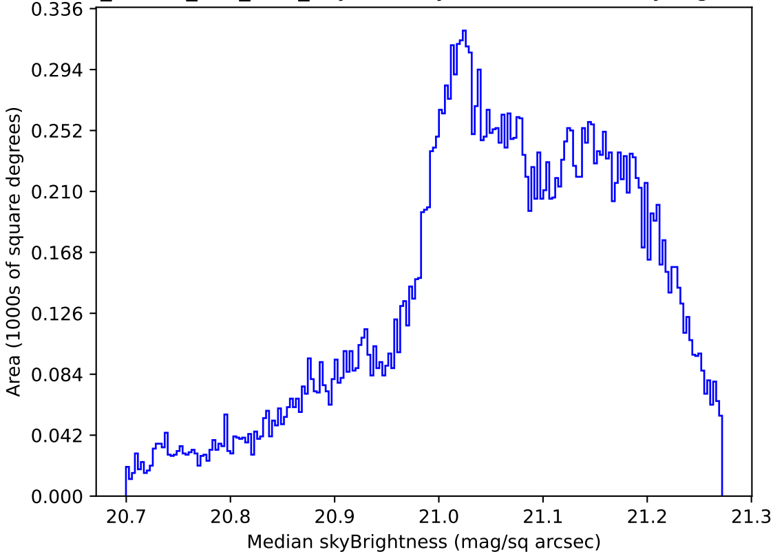
ddf_loaded_fl15_v3.4_10yrs All sky r band: Median skyBrightness
