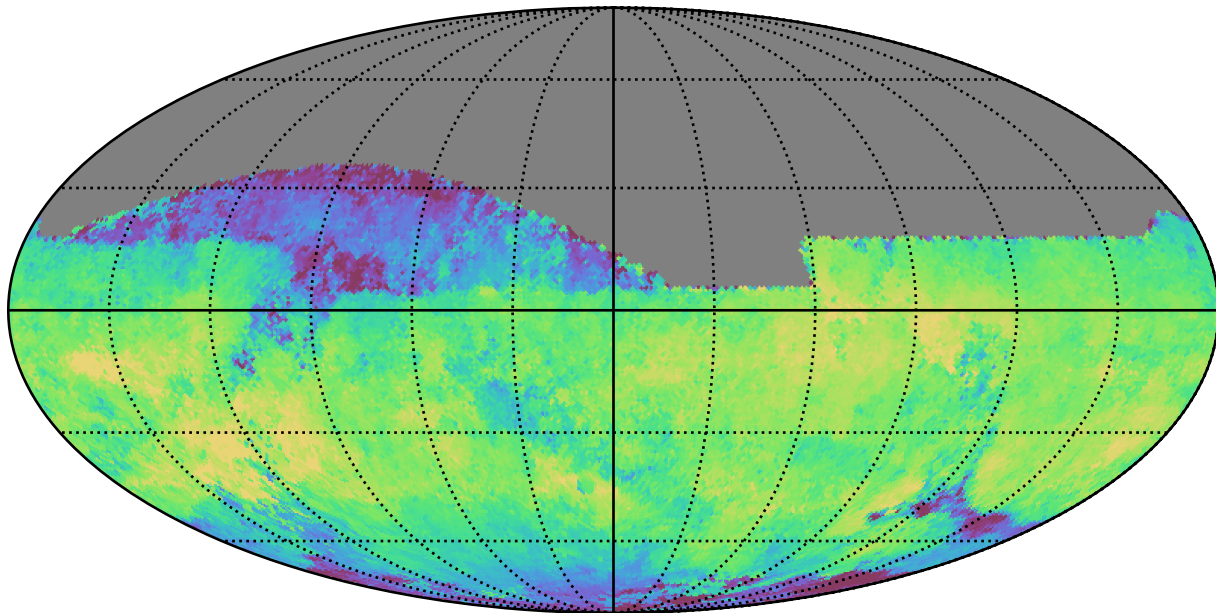
ddf_loaded_fl15_v3.4_10yrs All sky i band: Median skyBrightness
