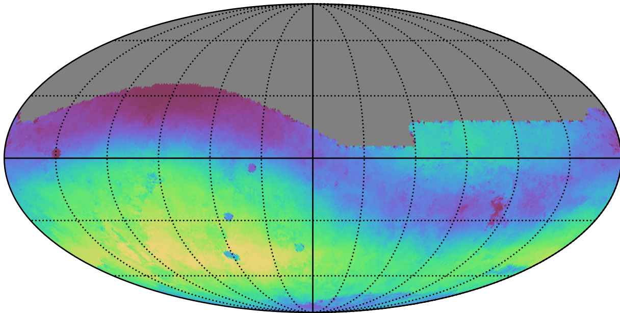
ddf_loaded_fl15_v3.4_10yrs All sky g band: Median skyBrightness
