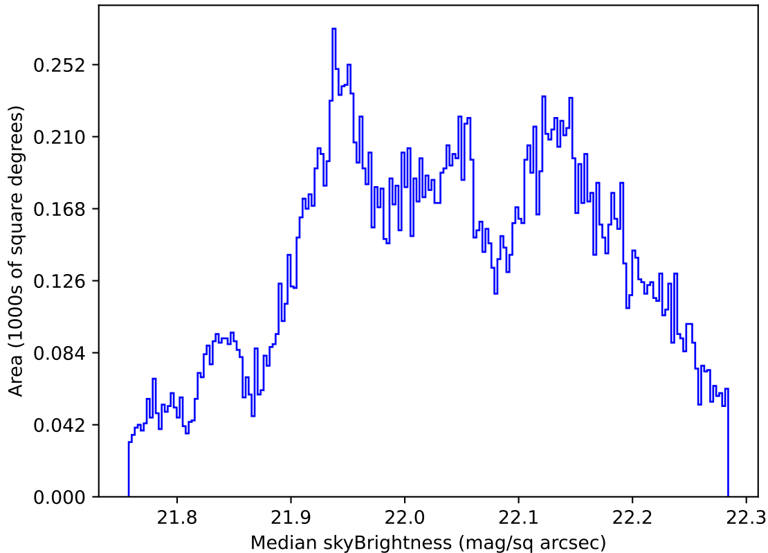
ddf_loaded_fl15_v3.4_10yrs All sky g band: Median skyBrightness
