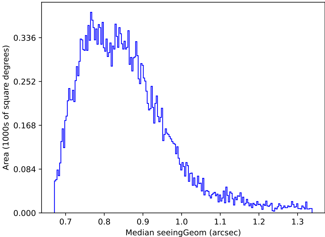
ddf_loaded_fl15_v3.4_10yrs Yr 1 z band: Median seeingGeom
