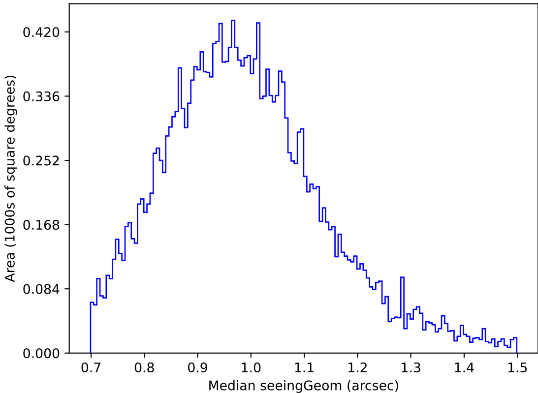
ddf_loaded_fl15_v3.4_10yrs Yr 1 u band: Median seeingGeom
